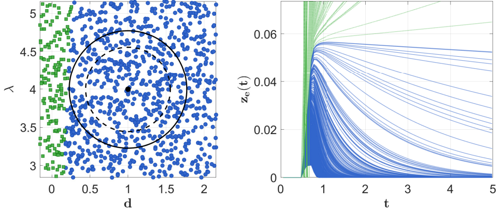
Fig. 4. Robust synthesis comparison. Left: stable (blue) and unstable (green) points with admissible uncertainty sets for structured (solid) and unstructured (dashed) synthesis. Right: trajectories for the structured observer gain using the same color coding. A step disturbance is applied for 0.5 \leq t \leq 0.75 .
